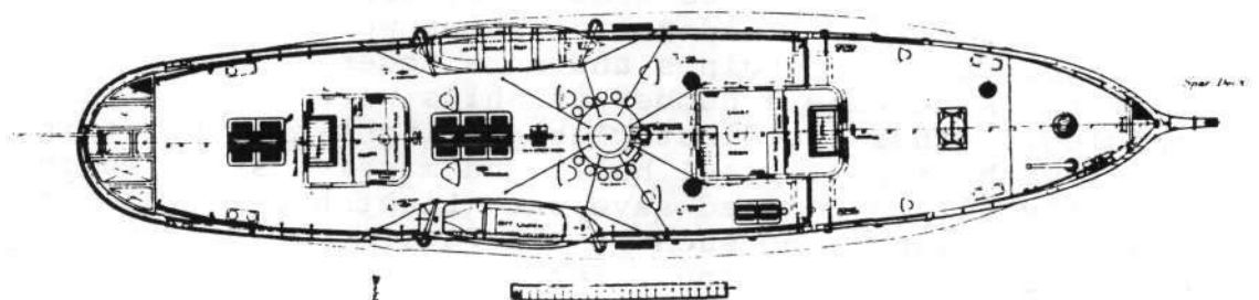
5. SECOND GENERATION STEEL-HULLED, STEAM-POWERED LIGHTSHIP NO. 94, SHOWN HERE, WAS TYPICAL FOR THE PERIOD 1904-1923. MANY OF HER SISTERS WERE LATER CONVERTED TO DIESEL AND DIESEL-ELECTRIC PROPULSION. (Society of Naval Architects and Marine Engineers)
