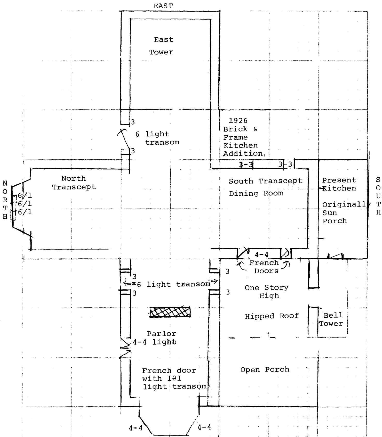
Figure 1 HO-353 Lilburn/Balderstone's Mansion First Floor Plan
